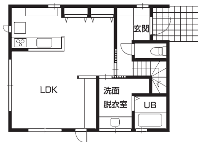
PLAN 1F
